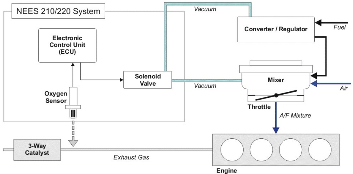
Figure 1. NEES 210/220™ Control System Schematic
