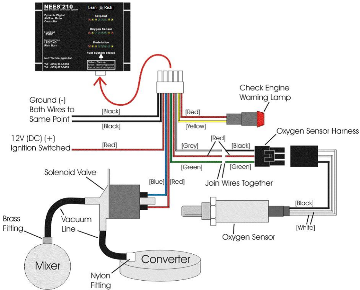
Figure 3. Electrical Connection Schematic
